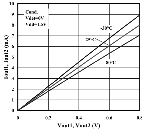
Iout vs Vout
