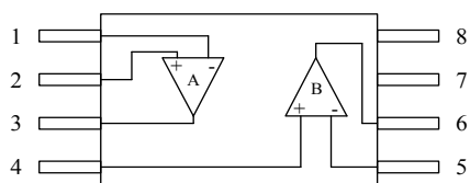
TSSOP-8(TOP VIEW)
