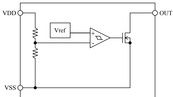
N-ch Output
