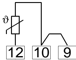
PT100 (RTD) 2-Wire
