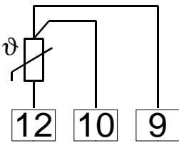
PT100 (RTD) 3-Wire
