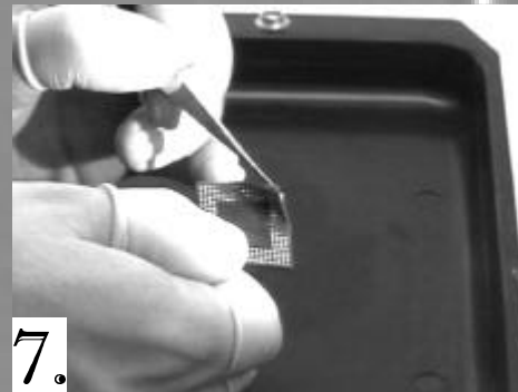
Remove the preform from the package
