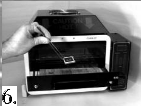
Reflow in oven
