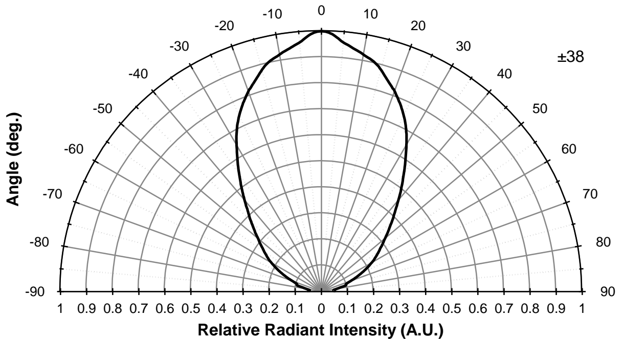
Radiation Characteristics
