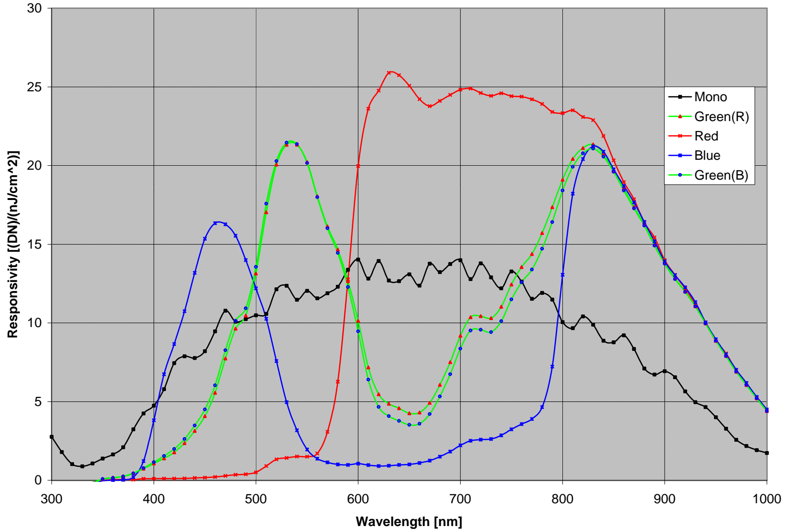
ZR32112 Spectral Response
