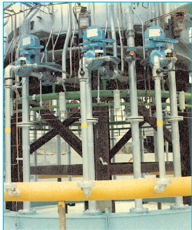
Air/gas supply pipes to vertical copper melting furnace (Continuus)
