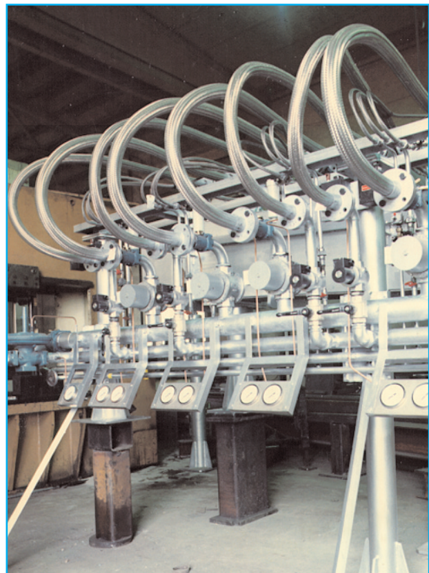
Lauder heating (Continuous)
