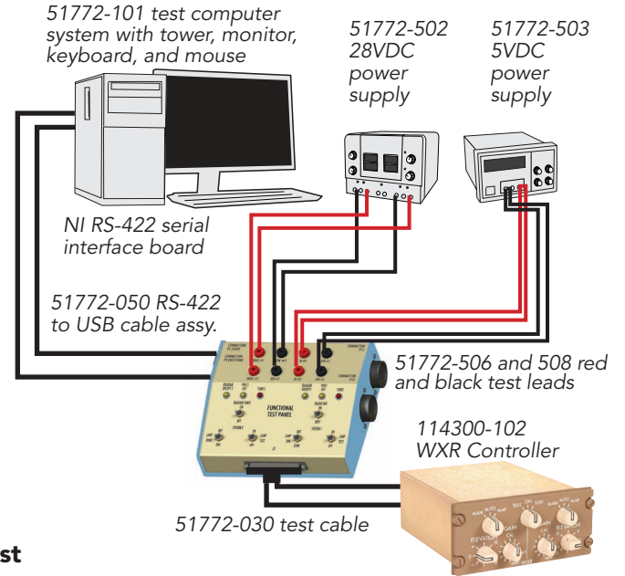
Figure 2 - Functional Test-Equipment Setup
