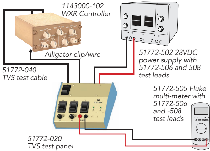
Figure 1 - TVS Test-Equipment Setup
