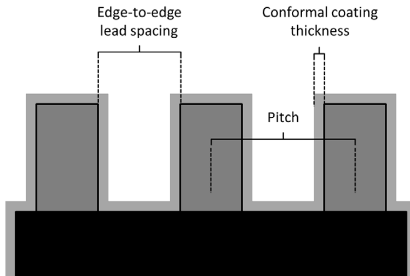
Figure 1: Diagram of conformal coated part geometries (from 41247 LFCEP Figure 2)
