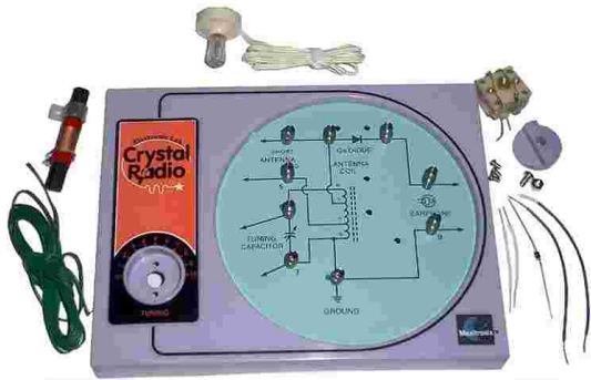
MX-901 Crystal Radio Kit AM.
