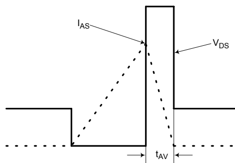
Figure 1. UIS Waveforms
