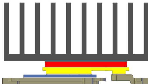
Figure 2: Cross section of Dual Cool and heat sink assembly.
