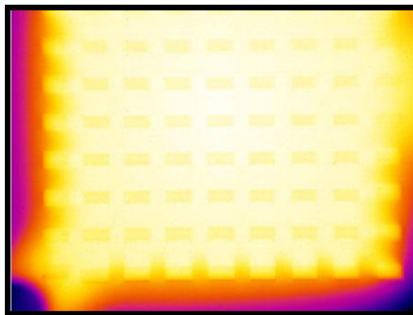
Figure 3: Thermograph of Dual Cool with heat sink in operation.
