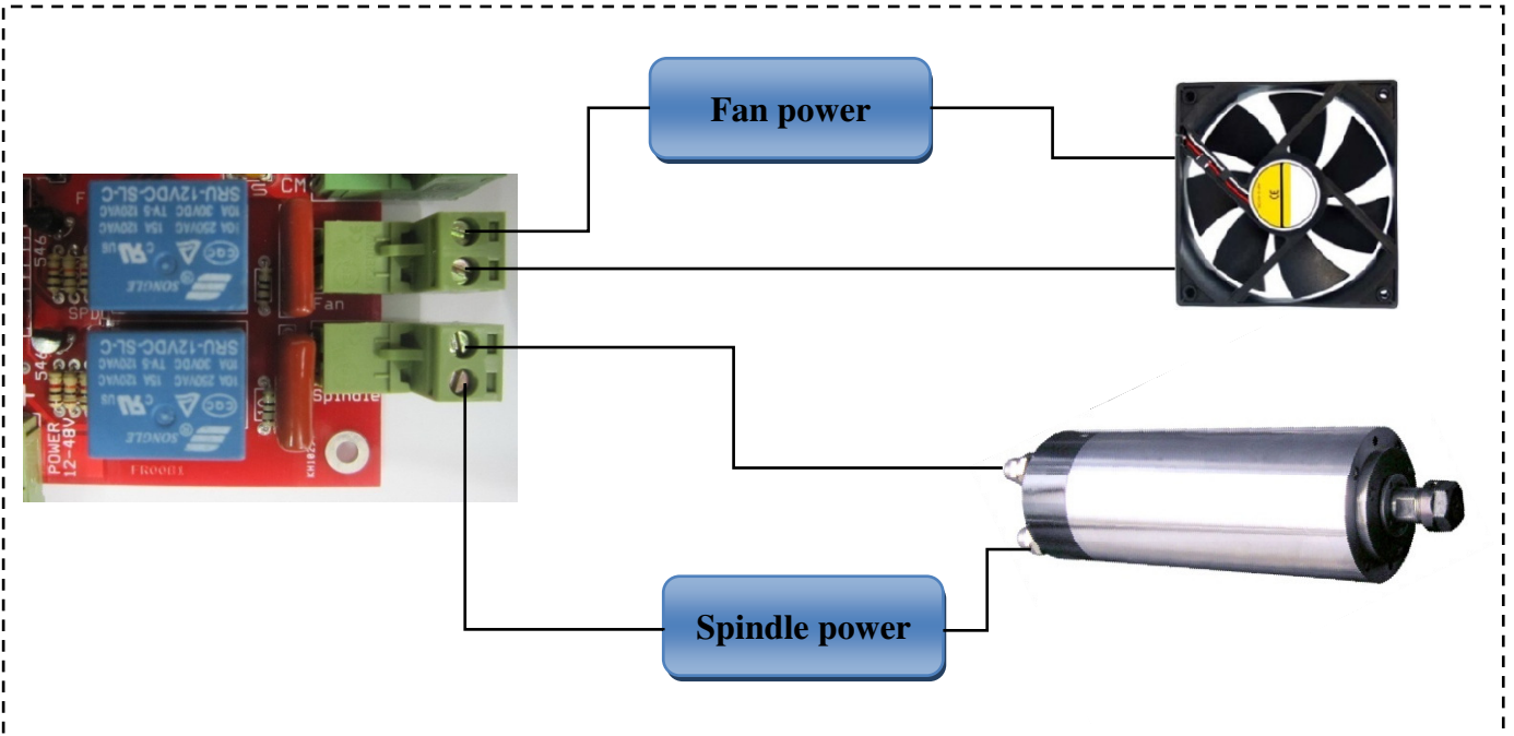
Figure 6. Connection of spindle motor and coolant fan to FIPBOB4
