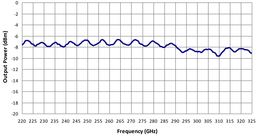
Typical FES-03 Output Power
