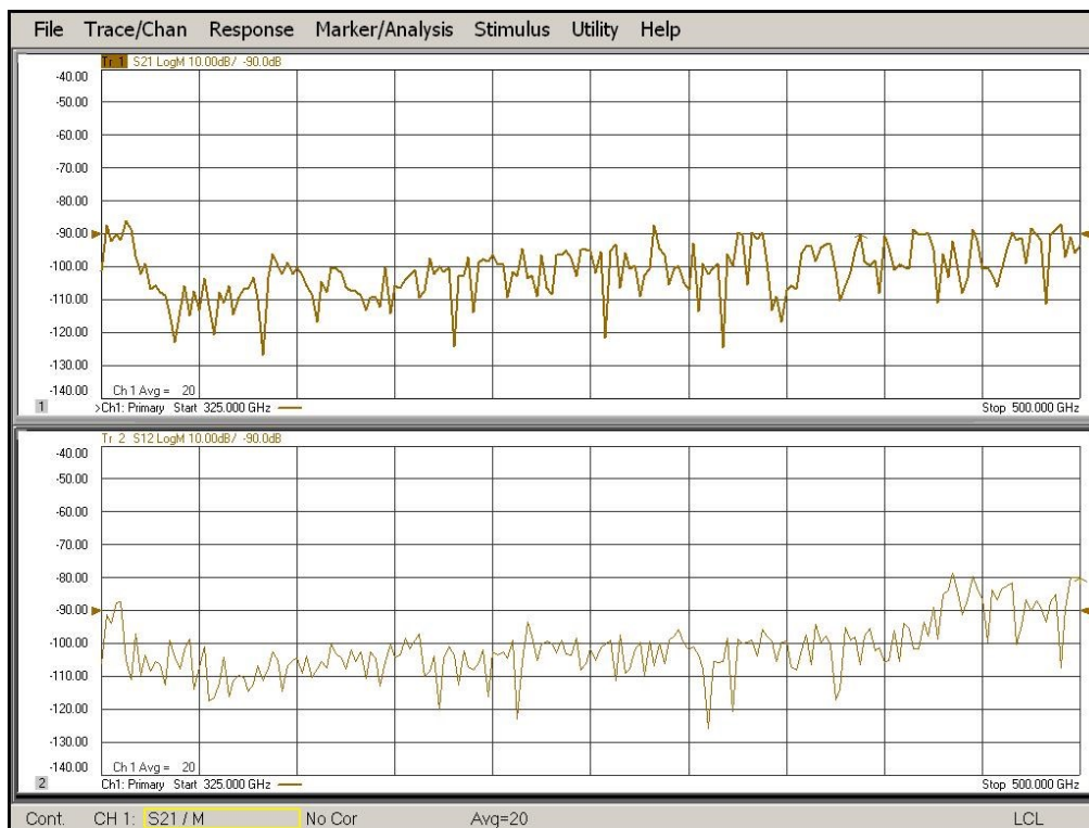
Figure 1. Typical FEV-02-TR system dynamic range.
