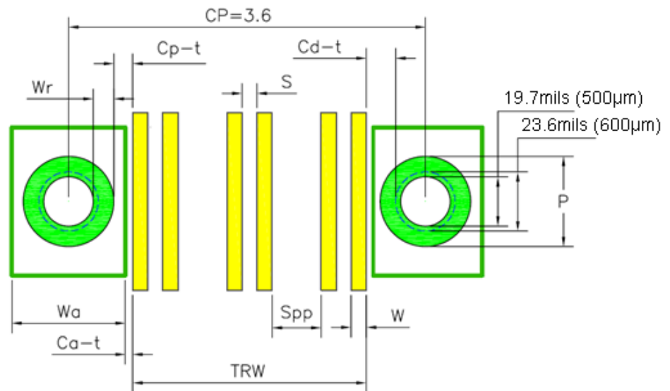
Two differential pairs per routing channel (Only 2 high speed signal layers required to route 6 differential pairs)
