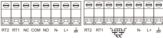
Relay output type(SPDT)
