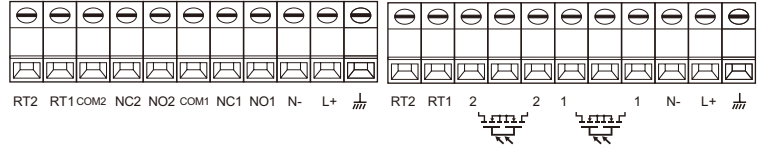
Relay output type (DPDT)
