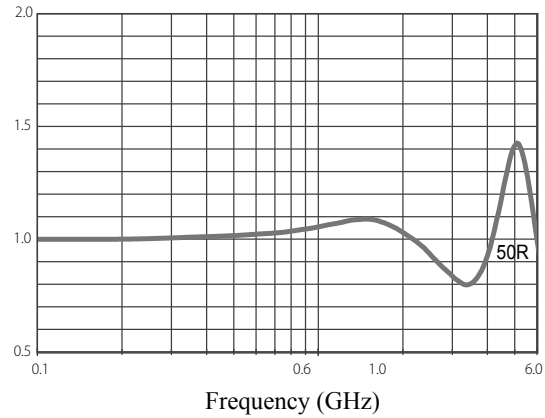
IZI/R for HFT201 MELF resistors
