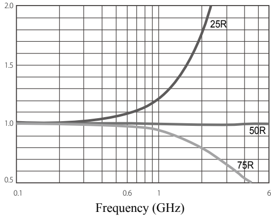
IZI/R for HFT204 MELF resistors
