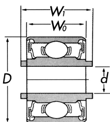
88000 Double Felt Seal
