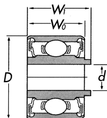
87000 Single Seal and Shield
