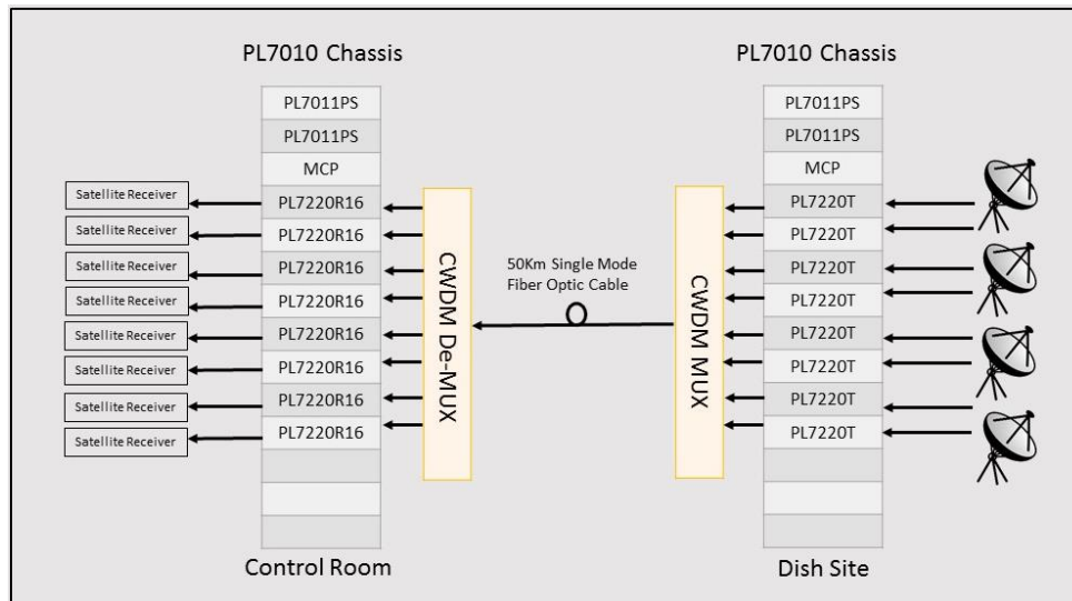
FIGURE 4: TYPICAL L-BAND SYSTEM
