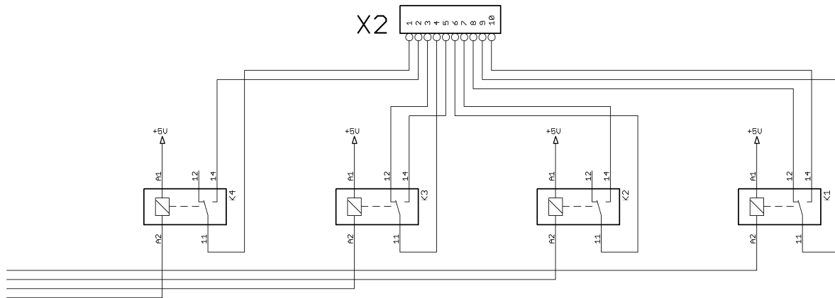
DIGITAL RELAY OUT 1 am Stecker X2
