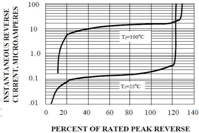
FIG. 3-TYPICAL REVERSE CHARACTERISTICS
