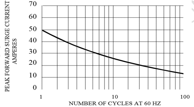
Fig. 4-MAXIMUM FORWARD SURGE CURRENT
