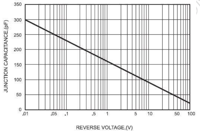
FIG.5-TYPICAL JUNCTION CAPACITANCE
