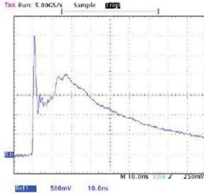
Fig3. ESD PULSE WAVEFORM, PER IEC 61000-4-2
