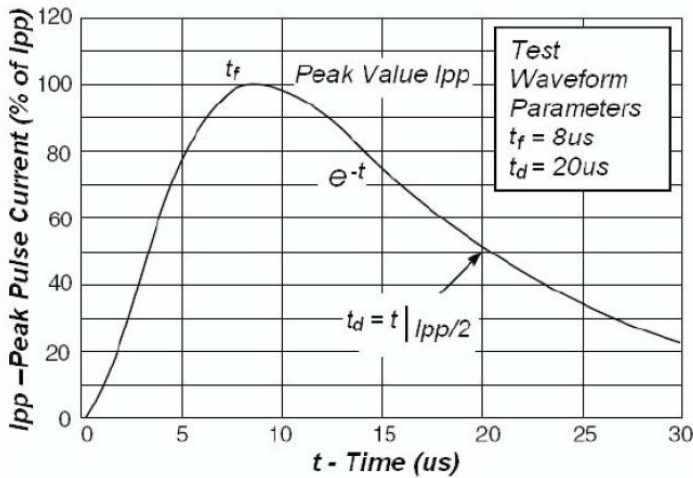
Fig1. Pulse Waveform
