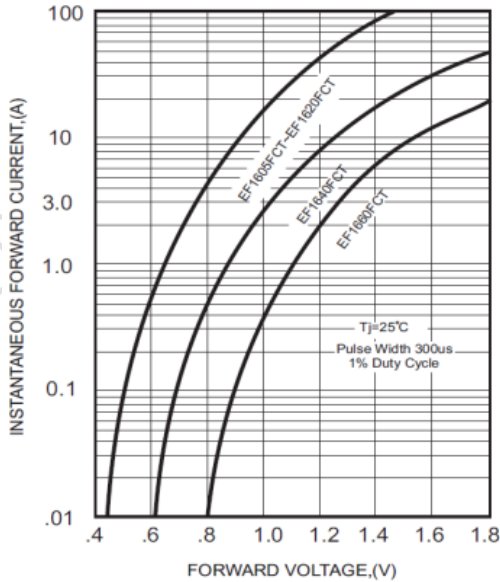
FIG.3-TYPICAL FORWARD CHARACTERISTICS
