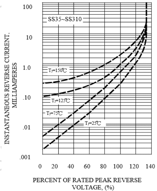
FIG. 3B - TYPICAL REVERSE CHARACTERISTICS
