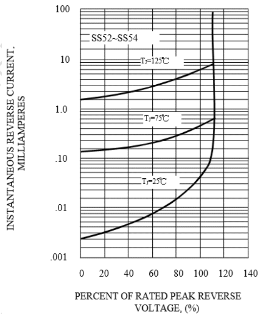
FIG. 3A - TYPICAL REVERSE CHARACTERISTICS
