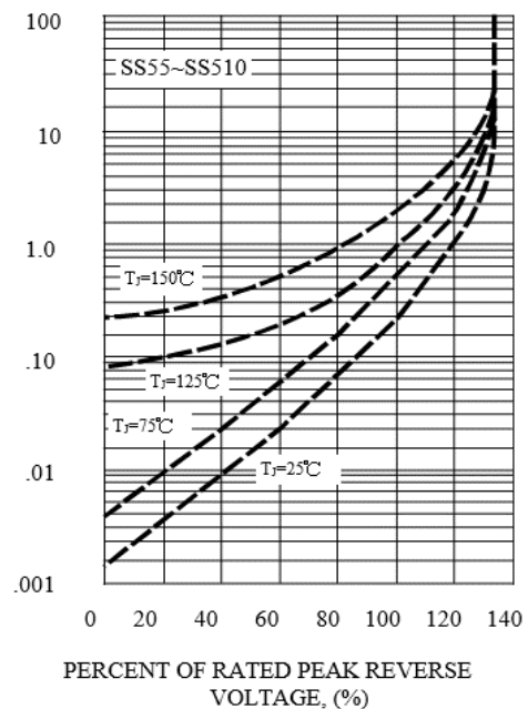
FIG. 3B - TYPICAL REVERSE CHARACTERISTICS
