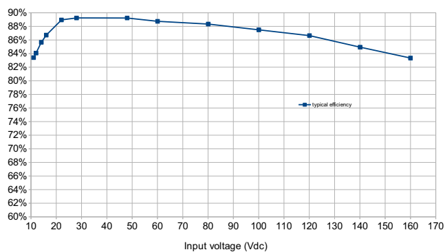
Typical Efficiency MGDD-20-R-I @ 25°C
