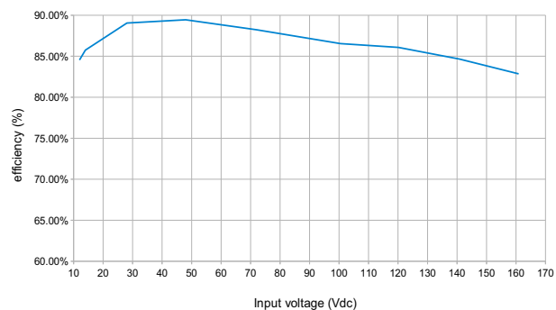
Typical Efficiency MGDD-20-R-E @ 25°C
