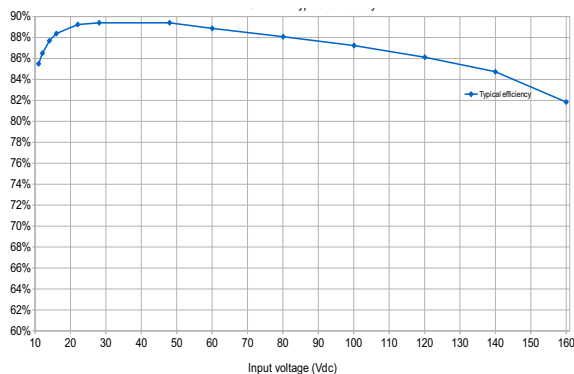
Typical Efficiency MGDD-20-R-F @ 25°C
