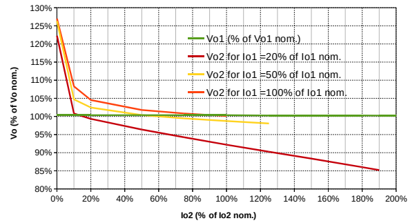
MGDD40N TYPICAL CROSS-REGULATION @ 25°C
