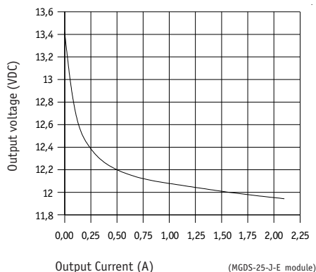
Figure 8 : Typical load regulation characteristics at nominal input
