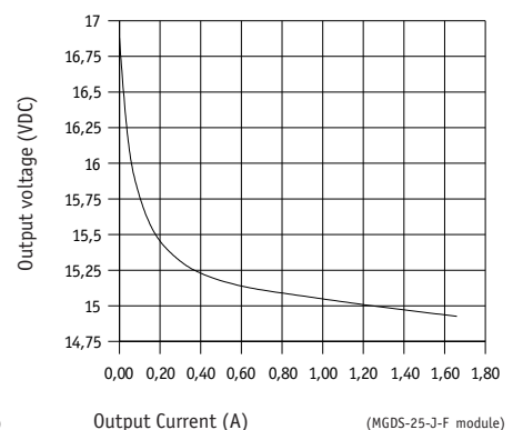
Figure 9 : Typical load regulation characteristics at nominal input
