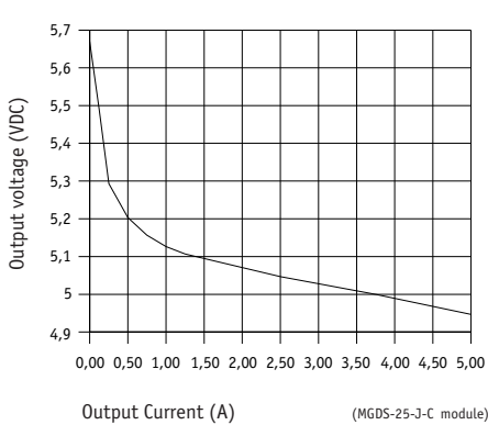
Figure 7 : Typical load regulation characteristics at nominal input
