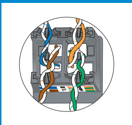
Pair Orientation for Cable End 2
