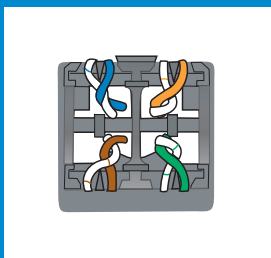
Pair Orientation for Cable End 1
