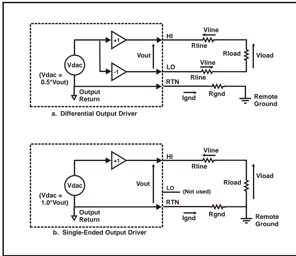
Figure 2.3-1. Output Configurations
