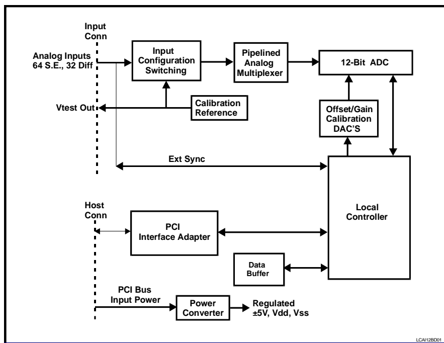
Figure 1.2-1. Functional Organization
