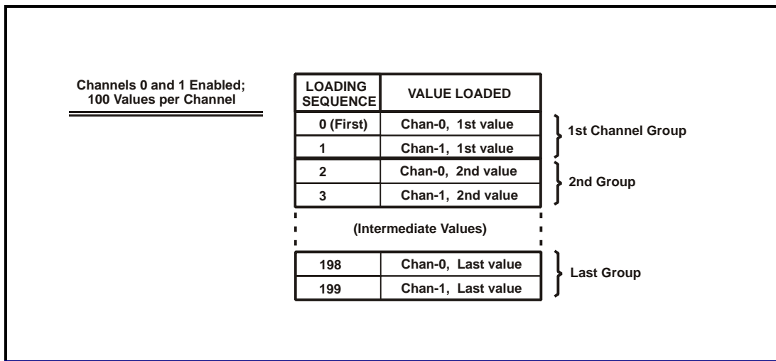
Figure 3.13-1. Typical Buffer Loading Sequence
