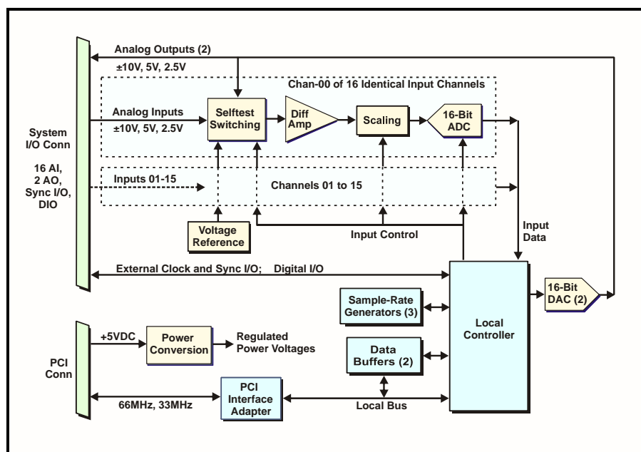
Figure 1.1-1. Functional Organization
