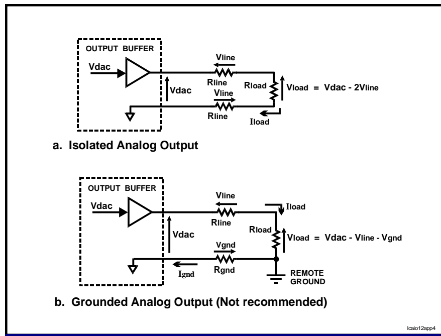
Figure 2.3-2. Output Configurations
