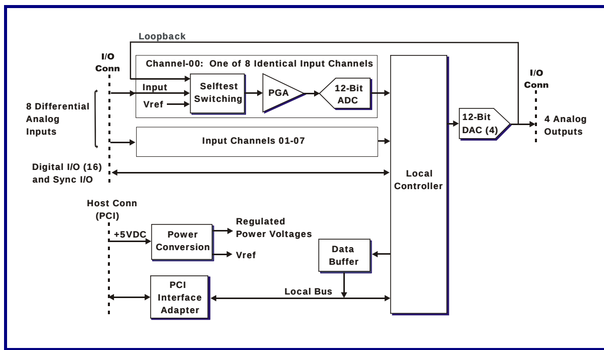
Figure 1.1-1. Functional Organization
