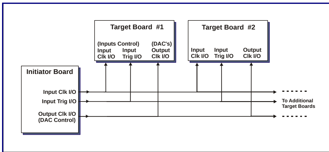
Figure 2.3-4. Multiboard Synchronization
