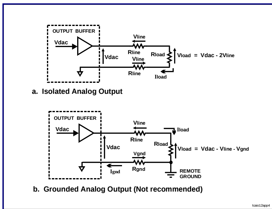
Figure 2.3-2. Output Configurations
