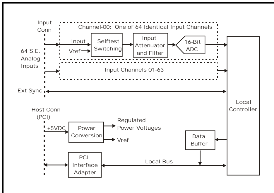
Figure 1.2-1. Functional Organization
