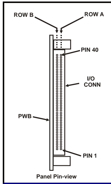
Figure 2.2-1. Input/Output Connector
