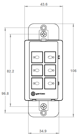
front view (Units in mm)
