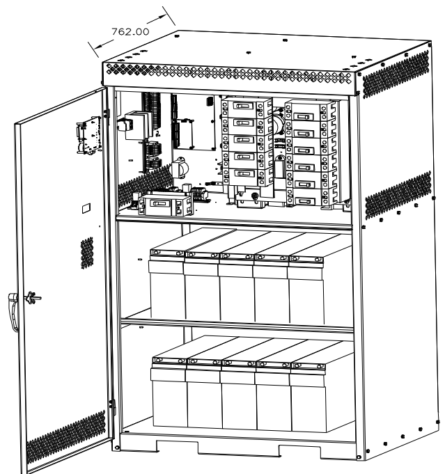
Cabinet RS3600-1 (see note 2, page 1) (BI configuration, single-row batteries)
