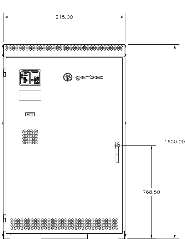
Cabinet RS3600-1 (see note 2, page 1) (BI configuration, single-row batteries)
