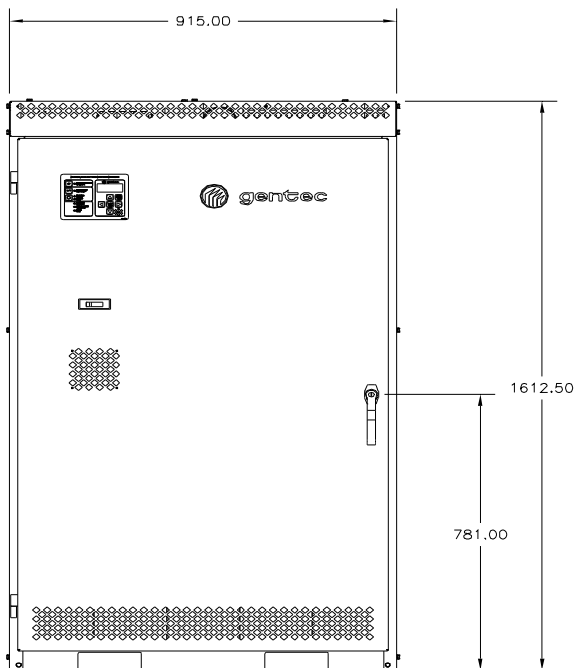
Cabinet RS3600-2 (see note 2, page 1) (BIP configuration, double-row batteries)
