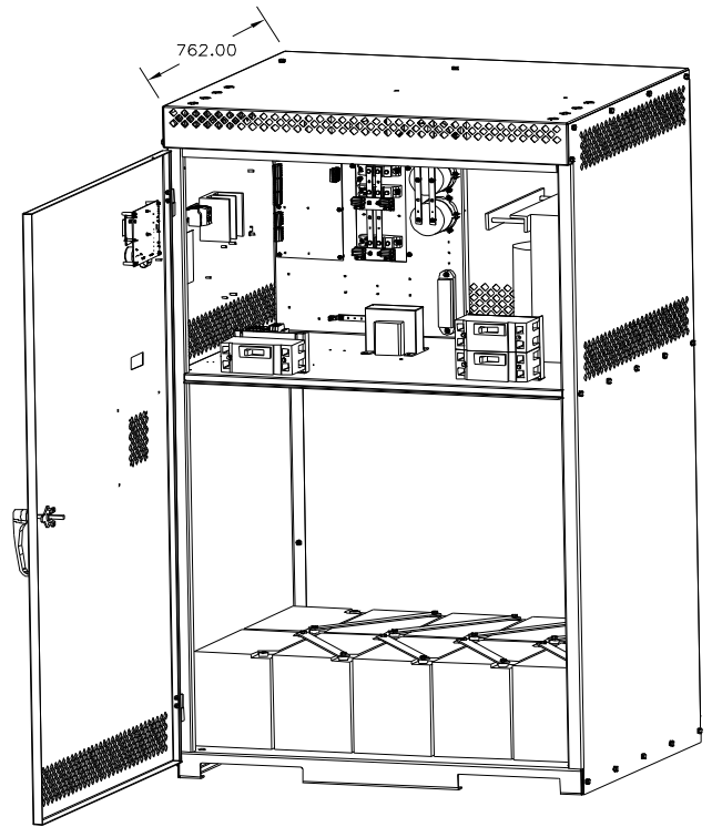
Cabinet RS3600-1 (see note 2, page 1) (BI configuration, single-row batteries)
