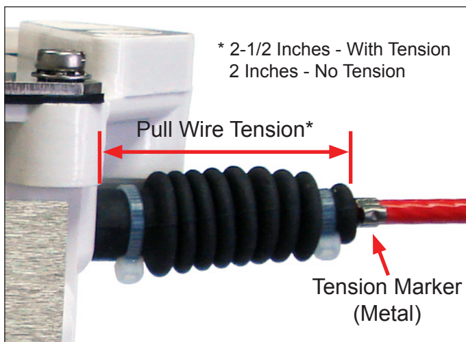
IMAGE C - Pull Wire Tension Indication
