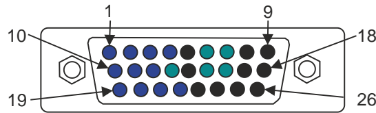
26-way HD Connector
