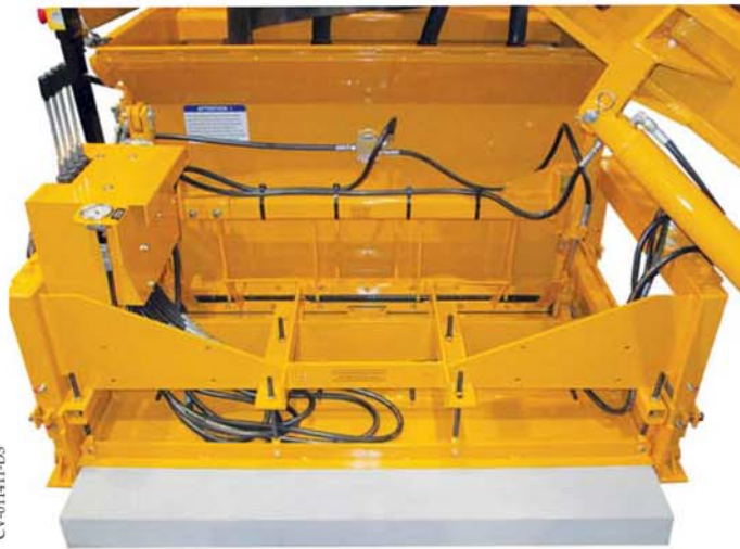
The mold on the GT-3200 sidewalk paver can be equipped with a hydraulic bar inserter and pressure-compensated sideplates.
