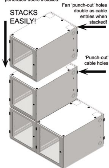
RCSC 12U, 36" deep cabinet shown here with optional perforated doors installed.
