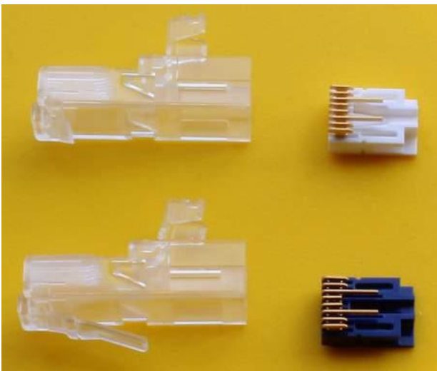
Old HARTING RJ Industrial® Gigalink Cat. 6 plug adapter and white and blue wire manager.
