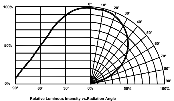
Relative Luminous Intensity vs. Radiation Angle
