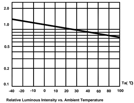
Relative Luminous Intensity vs. Ambient Temperature
