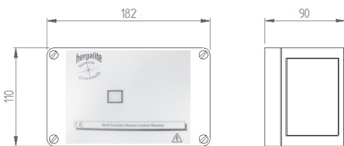
4 Channel Control Dimensions
