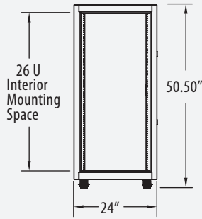
Front Elevation
