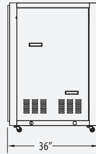
Side Elevation
