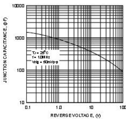
FIG. 3 - TYPICAL JUNCTION CAPACITANCE
