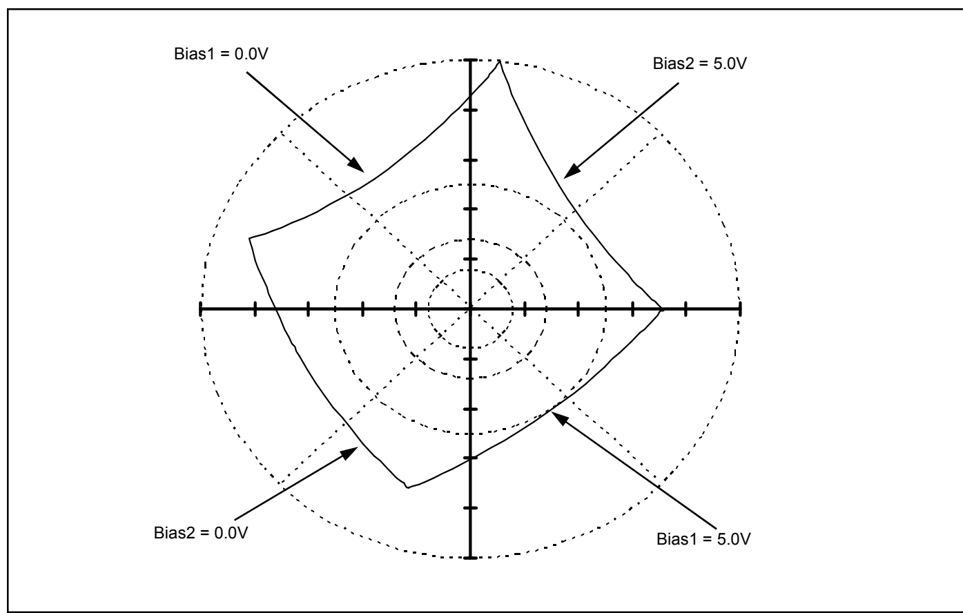
Figure 4. Transfer Function of Test to Determine Reference Loss
