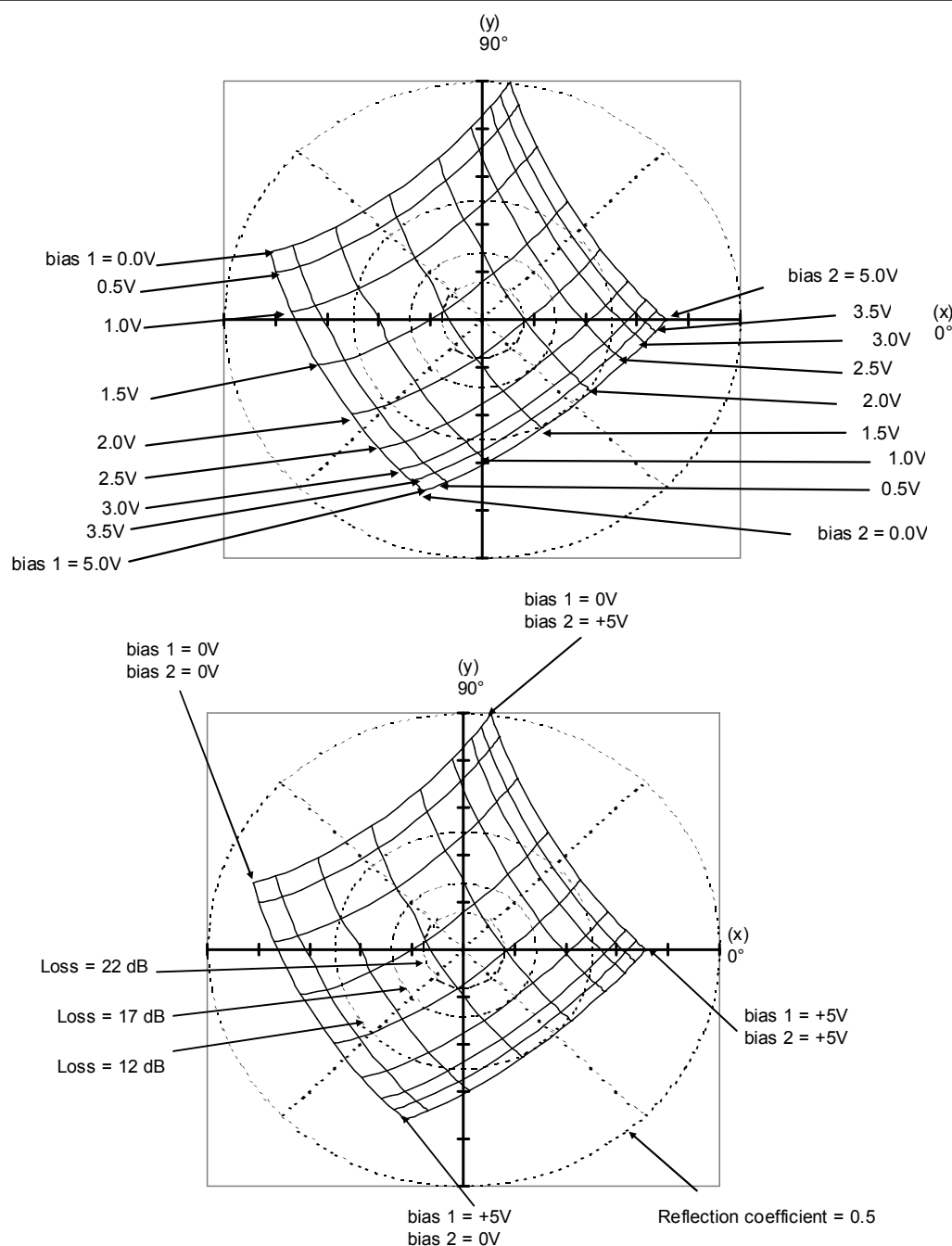
Figure 5. Phase and Attenuation of MAIA-007143-000100, Vector Modulator Linearized with MADR-007131-000100 Linearizer
