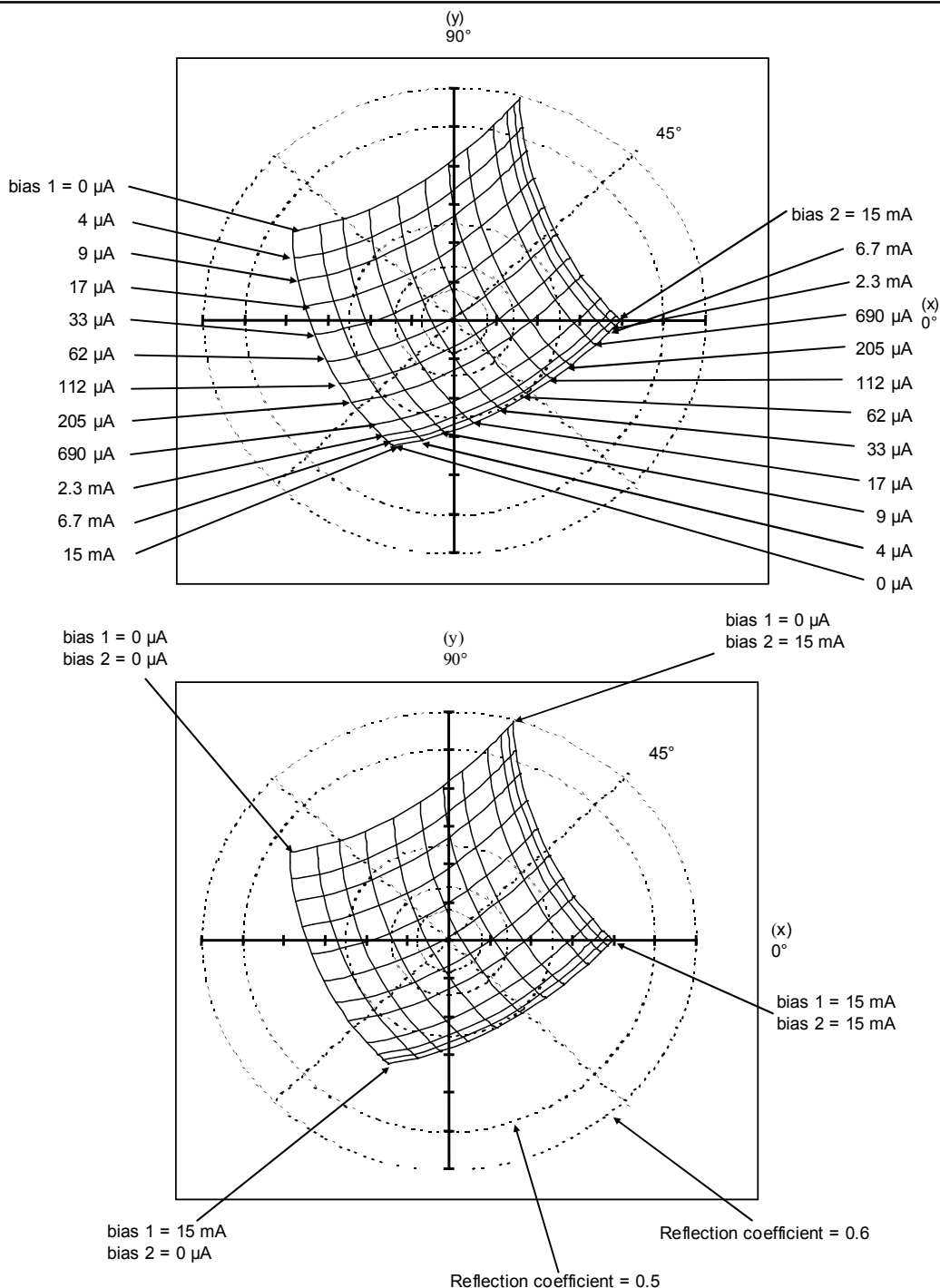
Figure 6. Phase and Attenuation of MAIA-007143-000100 vs. Bias Current
