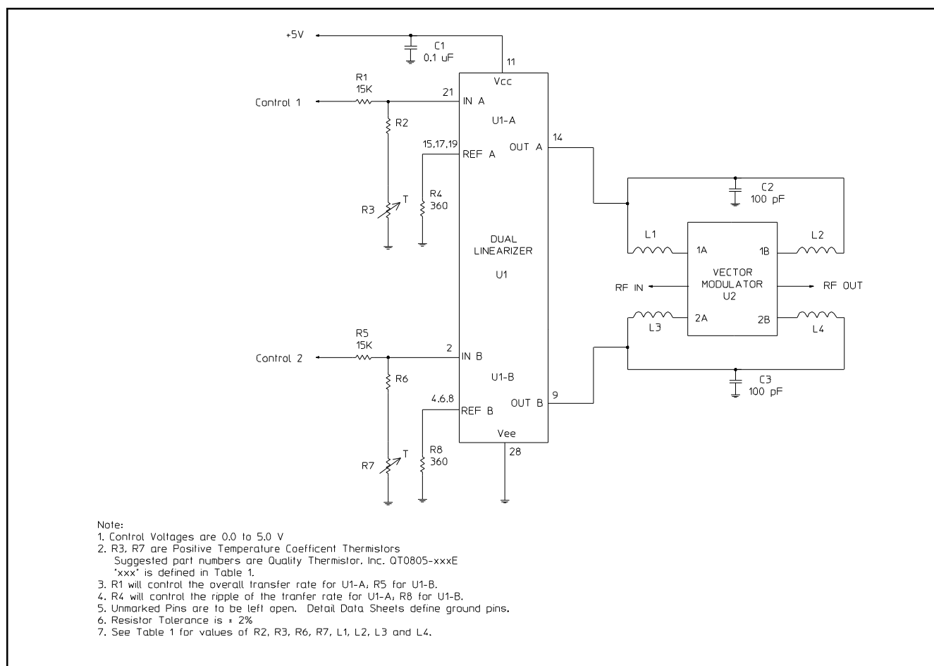
Figure 3. Schematic of Dual Linearizer Driving Vector Modulator
