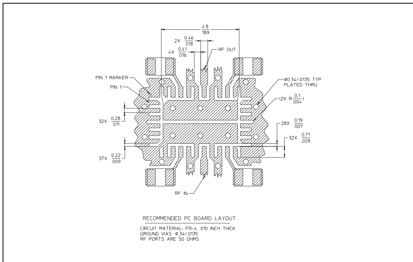
Figure 8. Recommended PC Board Mounting Pattern for Vector Modulators
